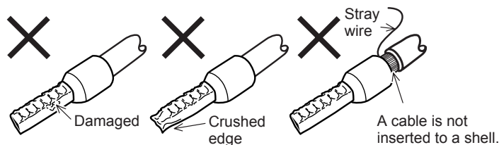
Figure 5.18 Example of incorrect bar terminal crimp
