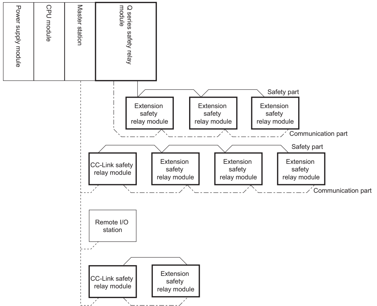
Figure 2.1 System configuration
