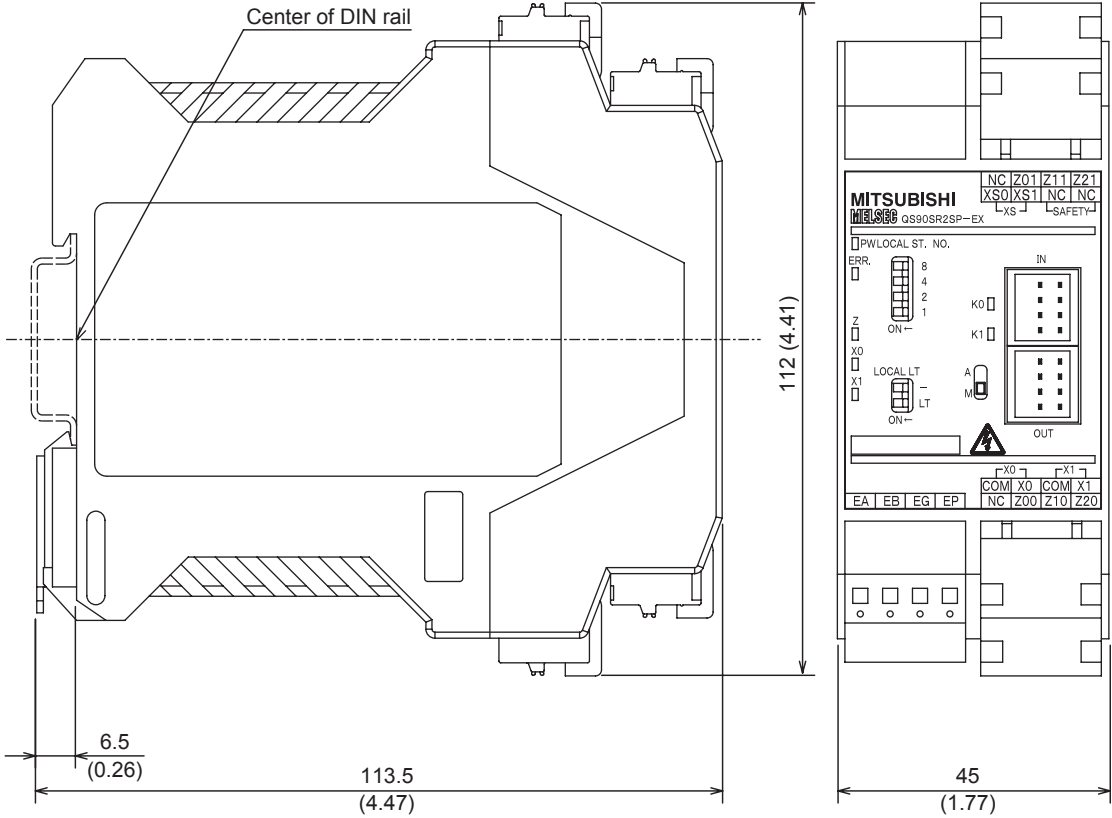
Figure App.3 QS90SR2SP-EX, QS90SR2SN-EX
