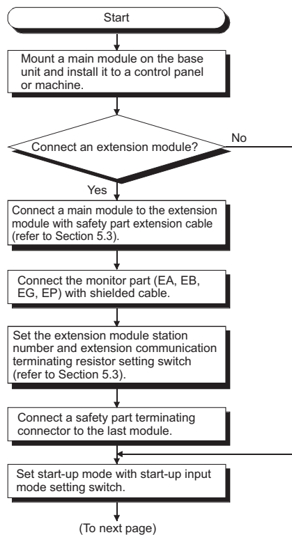
Figure 5.1 Start-up procedures (1/2)
